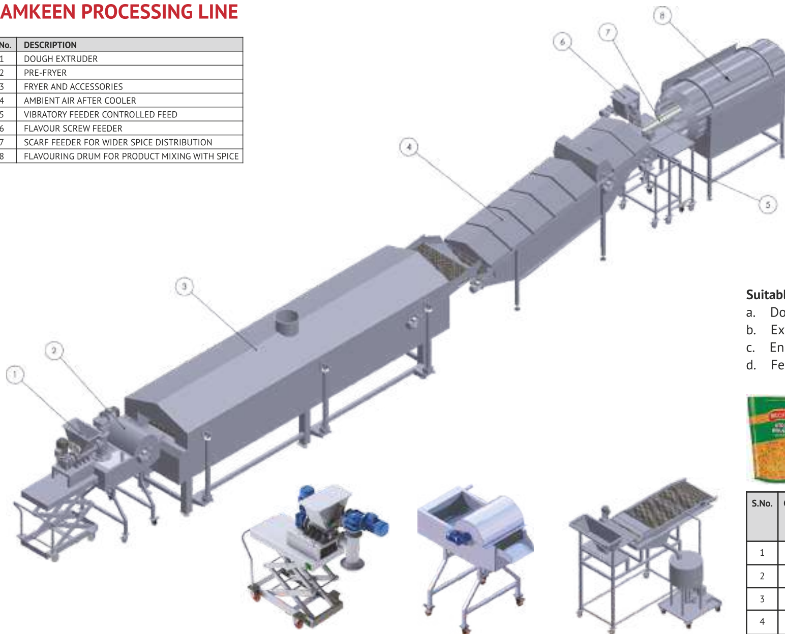
DOUGH EXTRUDER
